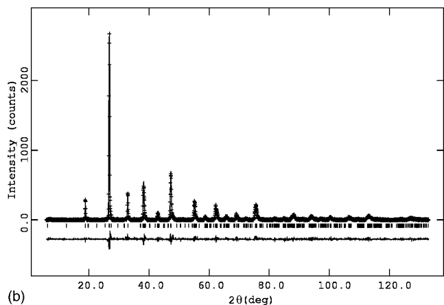
FIG. 2. (Color online) NPD (a) and SXPD (b) patterns of LBCCO fitted by the Rietveld method with the Pm\bar{3}m structural model described in Table I using GSAS/EXPGUI suite of programs.
